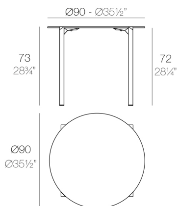
QUARTZ Mesa Ø90 QUARTZ Table Ø35 1/2"
